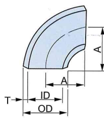
90°ELBOW (SHORT)
