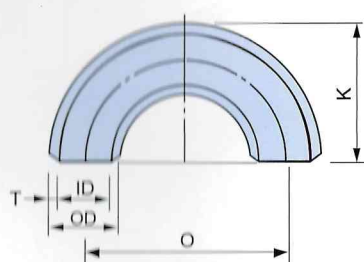
180°ELBOW (LONG)
