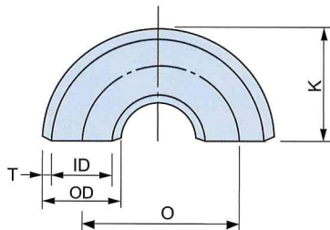
180°ELBOW (SHORT)
