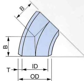
45°ELBOW (LONG)
